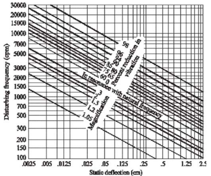
Figure 9. Isolation Efficiency of Resiliently Mounted System.
