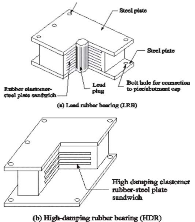
Figure 13. Seismic Isolation Devices.
