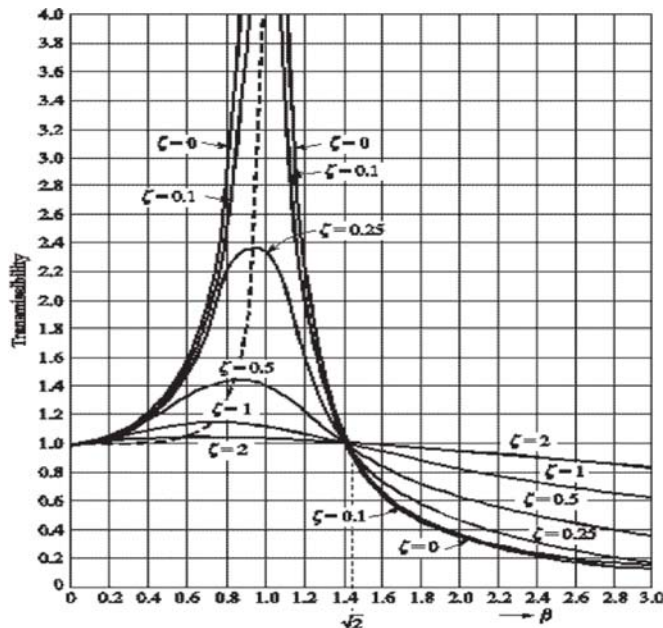
Figure 10. Variation of Transmissibility ( Tr ) with Frequency Ratio for Steady State Dynamic Loading.
