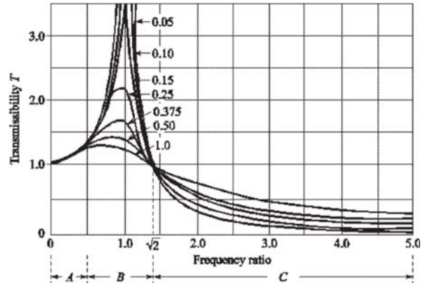
Figure 2. Range of frequency ratio for vibration isolator ( Tr s Vrs frequency ratio).
