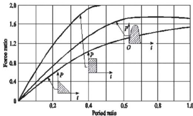
Figure 11. Variation of Transmissibility with Period Ratio for Pulse Loadings.
