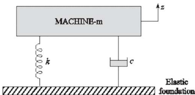
Figure 1. Machine supported on elastic foundation.
