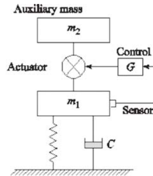
Figure 4. Schematic Diagrams for Active Control System.
