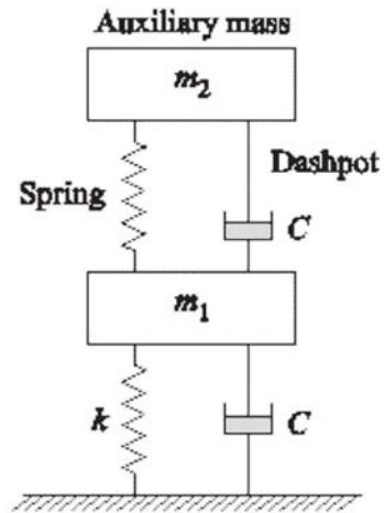
Figure 5. Schematic Diagrams for Passive Control System.
