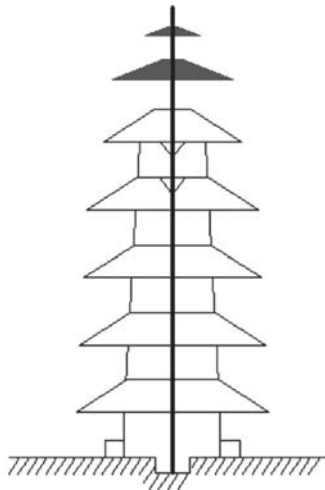
Figure 3. Wooden pagoda with suspended pole that is free to oscillate. (After Tanabashi, R, 1960).
