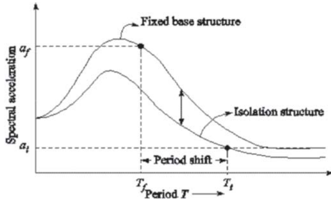
Figure 12. Response of a Fixed Base and Isolated Structure.
