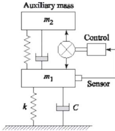
Figure 6. Schematic Diagram for Hybrid Control System.
